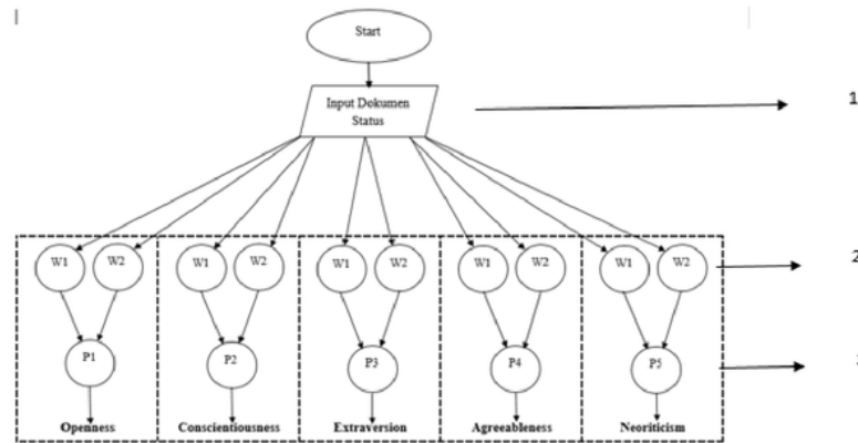
Fig.3. Probabilistic Neural Network Flow
